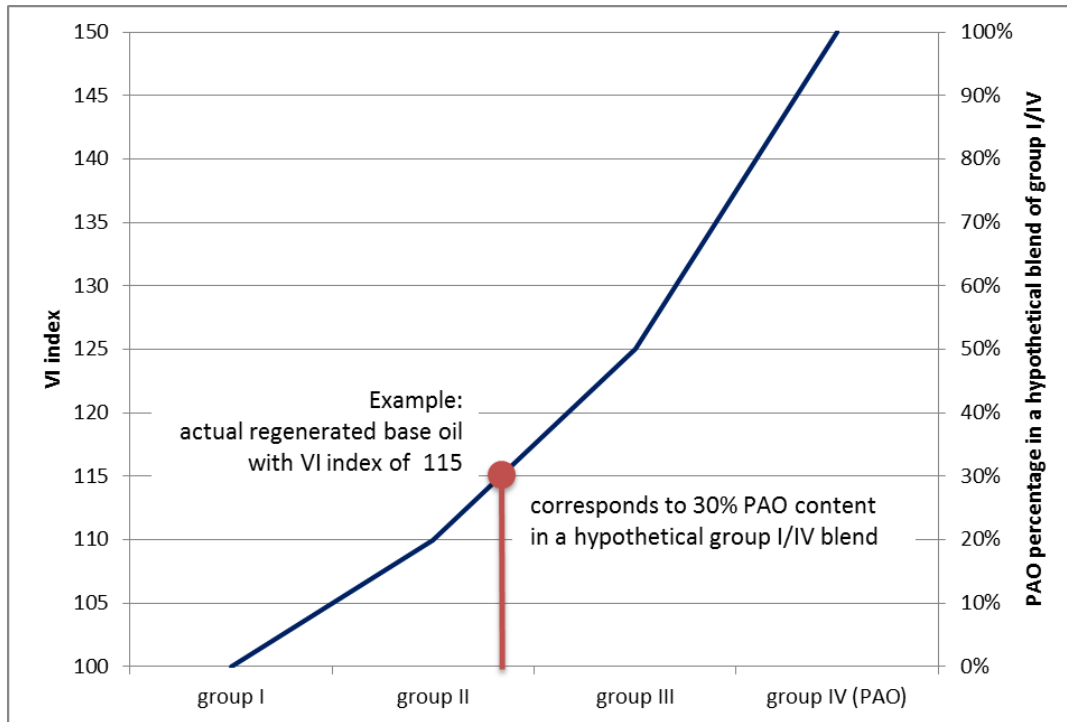
Figure 2: Correlation model based on viscosity index (VI) by actual recycled base oil as a numerical indication for the definition of replaced virgin base oil hypothetically blended from group I and group IV base oil.
