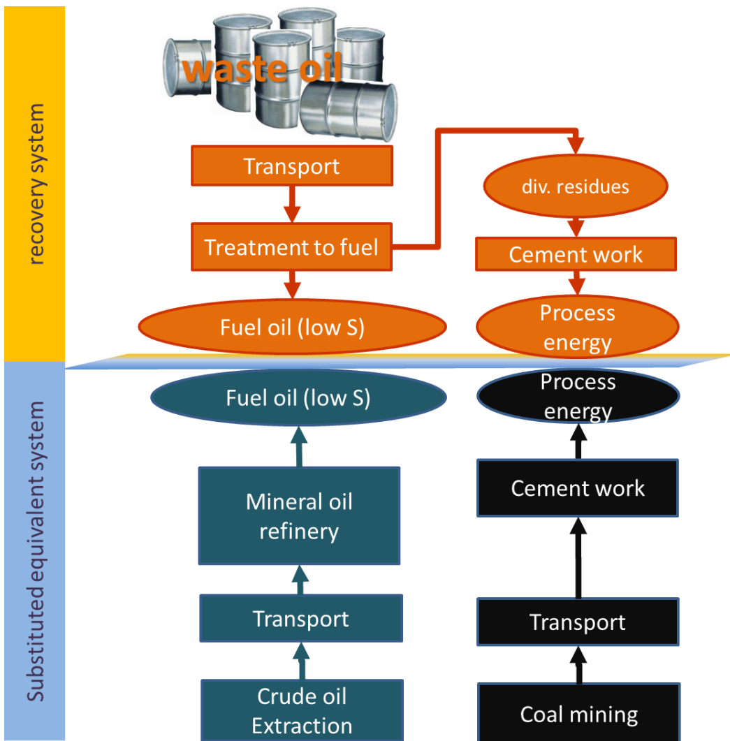
Figure 4: Simplified scheme of the system boundary for the reference system and its substituted equivalent system
