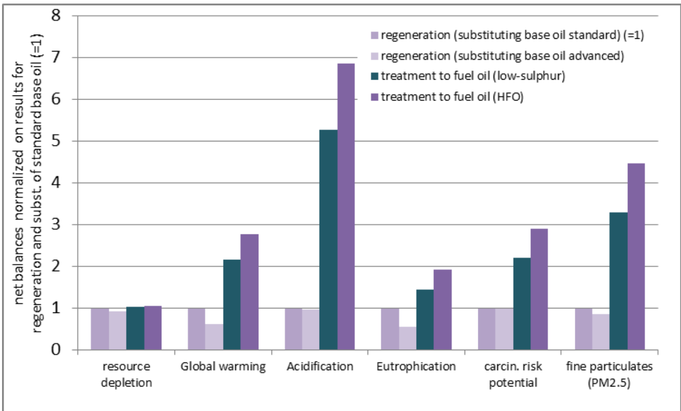
Figure 17: Total view on the comparable impact assessment results – regeneration (average) vs. treatment to fuel – sensitivity of the choice of fuel oil type - ; values <1 describe better performance than regeneration (base oil group I) and vice versa.
