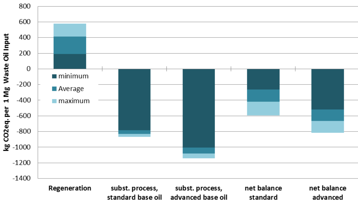
Figure 8: Impact assessment results for global warming; showing the average result (arithmetic mean) of the four techniques as well as the individual minimum and maximum
