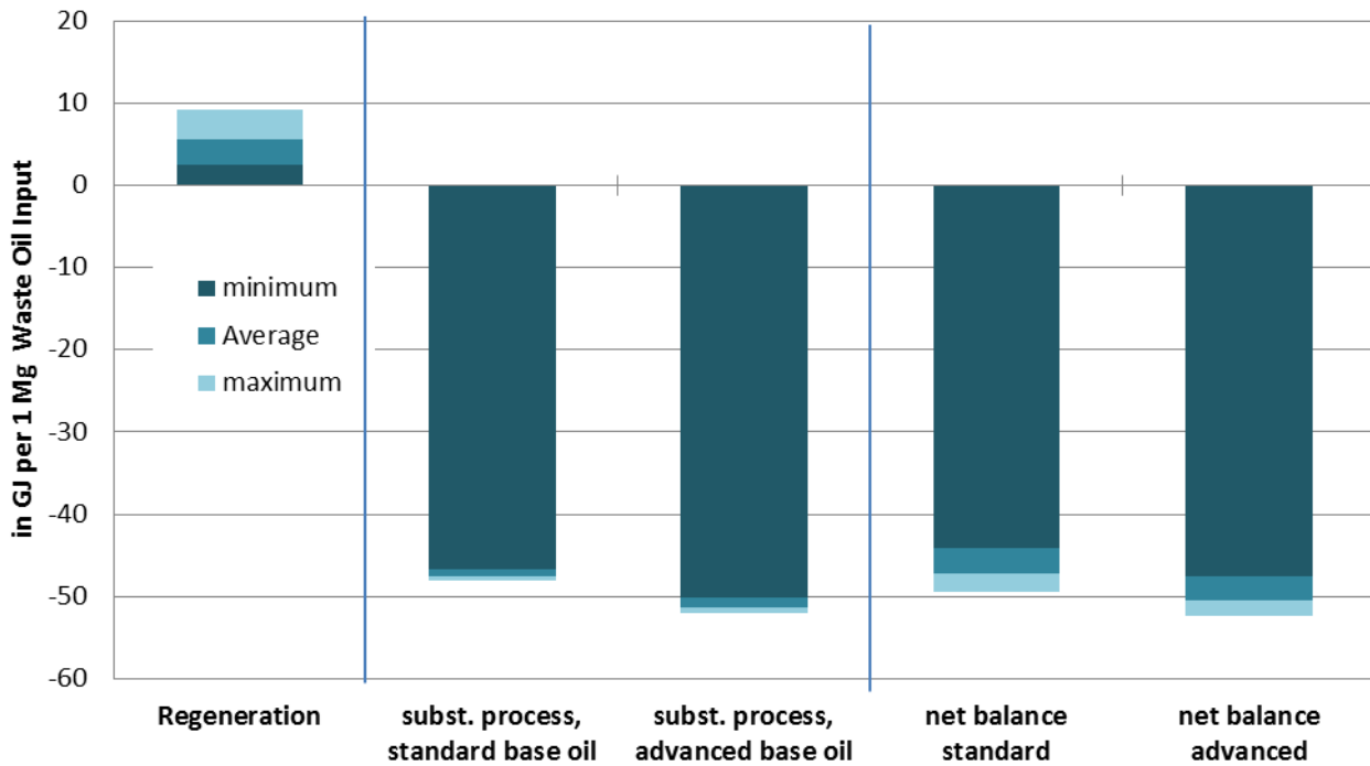
Figure 7: Impact assessment results for resource depletion; showing the average result (arithmetic mean) of the four techniques as well as the individual minimum and maximum.
