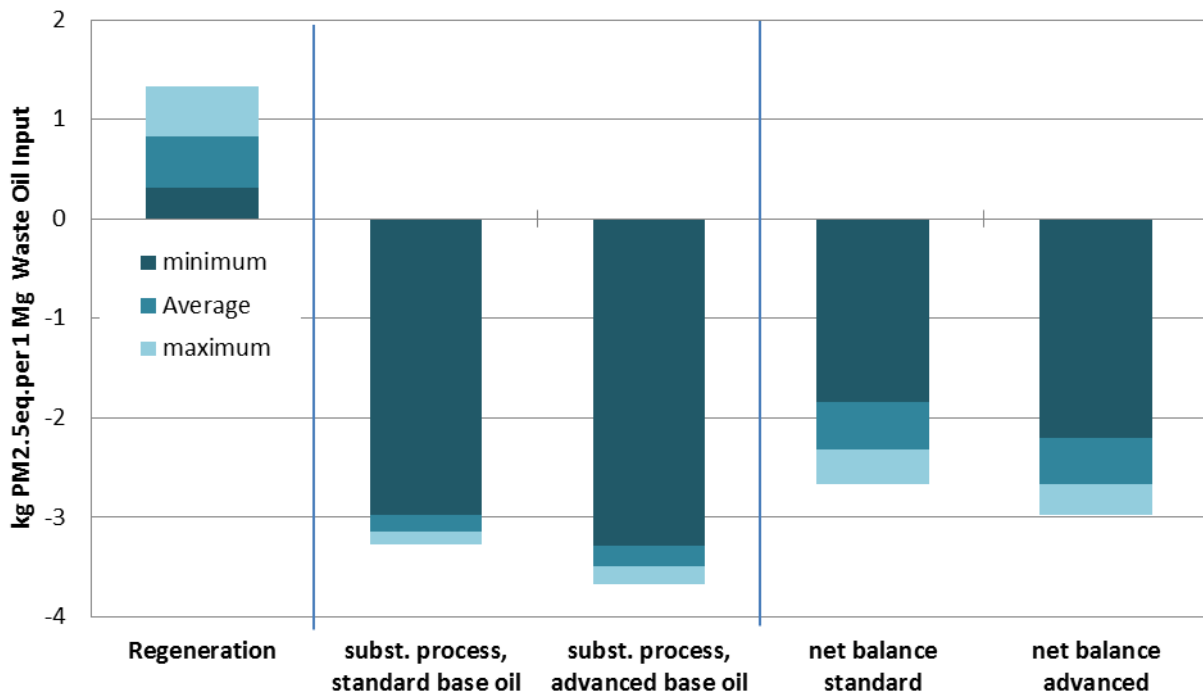
Figure 12: Impact assessment results for human toxicity represented by fine particulates (PM2.5 showing the average result (arithmetic mean) of the four techniques as well as the individual minimum and maximum.
