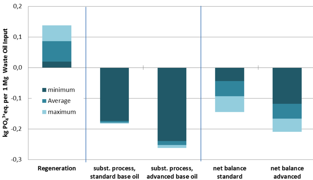
Figure 10: Impact assessment results for eutrophication; showing the average result (arithmetic mean) of the four techniques as well as the individual minimum and maximum
