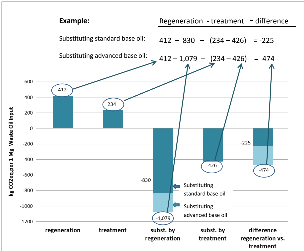
Figure 14: Illustrative example for the final combination of the impact assessment result to analyze the difference between regeneration and treatment to fuel oil.
