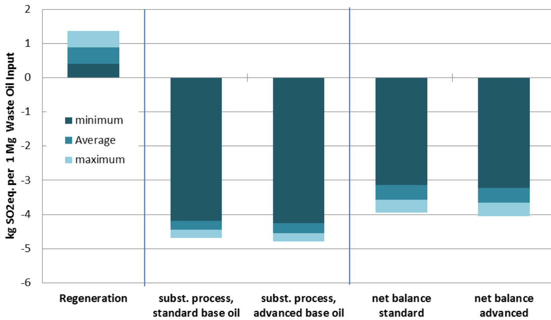
Figure 9: Impact assessment results for acidification; showing the average result (arithmetic mean) of the four techniques as well as the individual minimum and maximum
