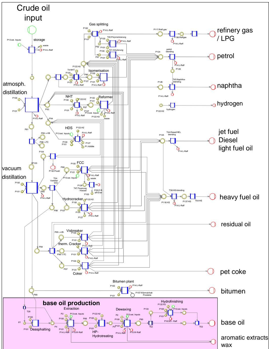
Figure 6: Network model for the calculation of mass and energy flow of a virtual mineral oil refinery
