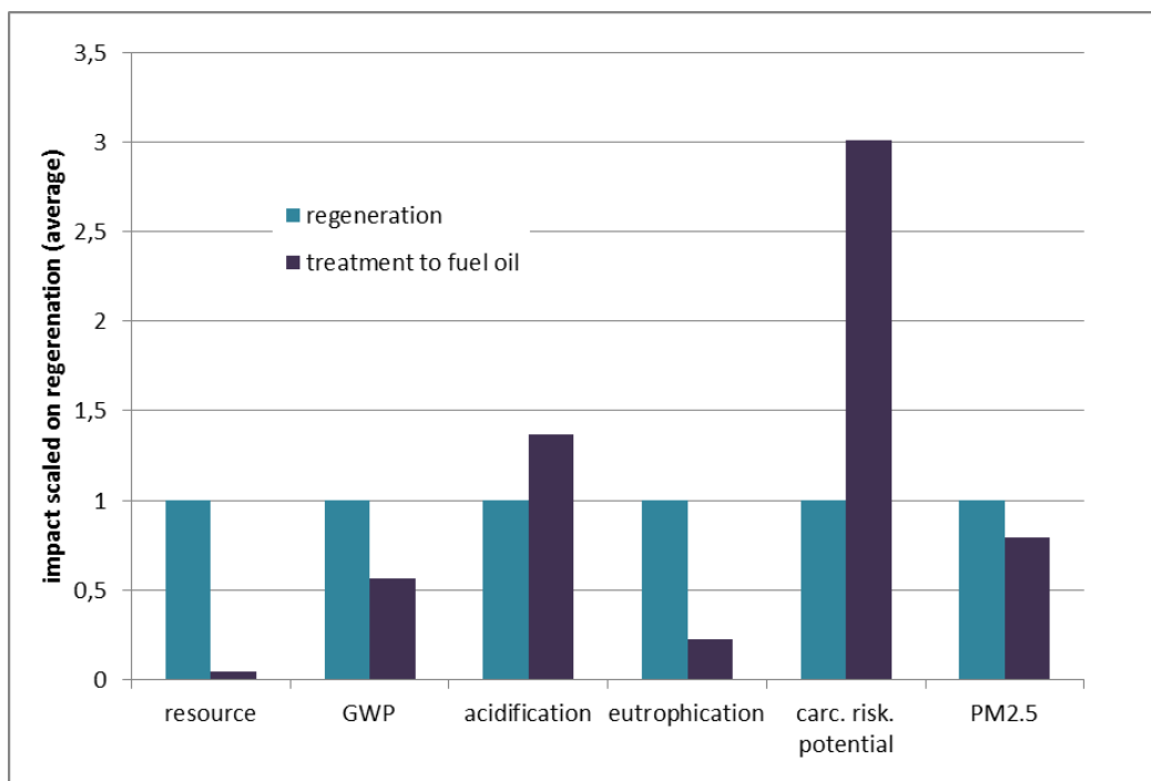
Figure 18: Comparison of regeneration (average) and treatment processes (no substituted equivalency system considered) scaled on regeneration for each impact category.
