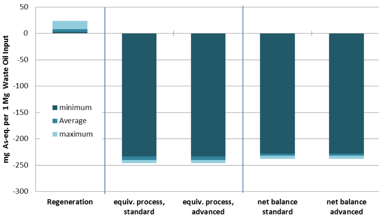
Figure 11: Impact assessment results for human toxicity represented by carcinogenic risk potential; showing the average result (arithmetic mean) of the four techniques as well as the individual minimum and maximum
