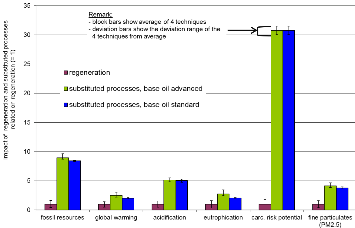
Figure 13: Total view on the impact assessment results; all figures related to the particular result of “regeneration”, main bars: average result (arithmetic mean) of the four techniques, deviation bars: range of the four techniques
