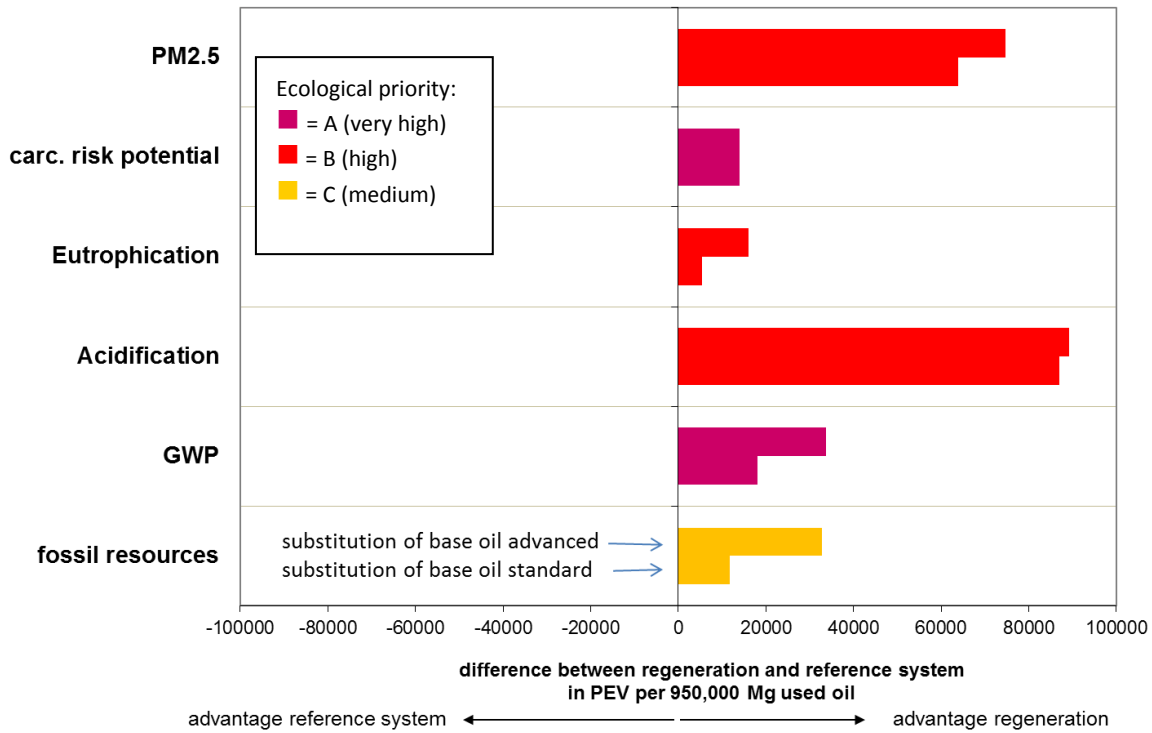
Figure 16: Overview of impact-related and normalized differences between average regeneration and treatment to fuel oil
