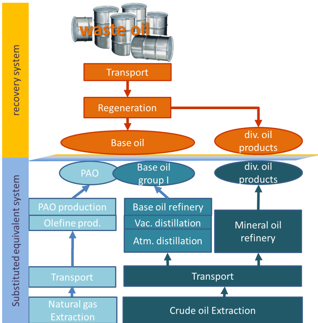
Figure 3: Simplified scheme of the system boundary for regeneration and its substituted equivalent system
