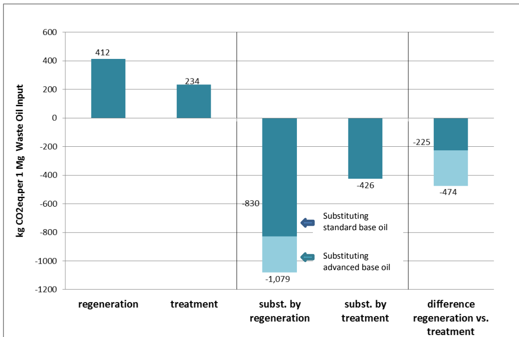
Figure 20: GWP for regeneration, treatment and its equivalency systems and final combination of these components for the comparison of both options.
